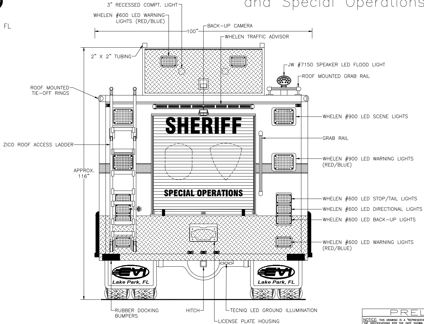
Rear View
