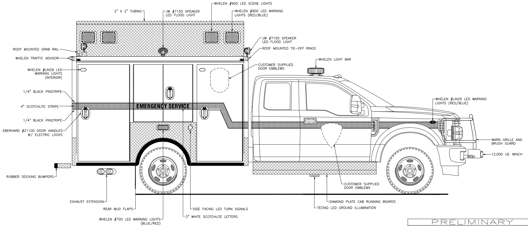
Curbside Overall
