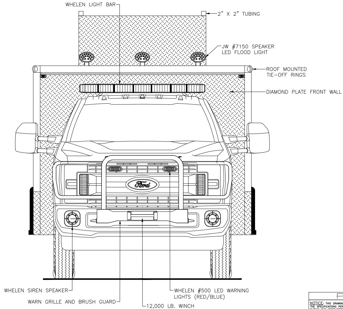
Front View
